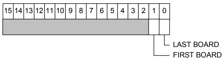
Fig. 4.20: MCST Address Register
