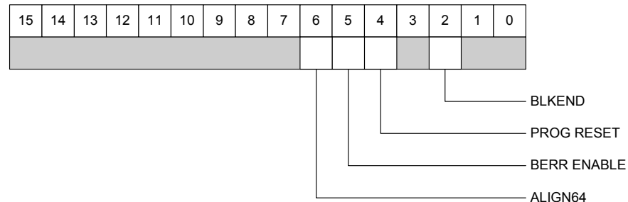
Fig. 4.17: Control Register 1
