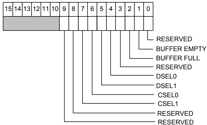
Fig. 4.21: Status Register 2
